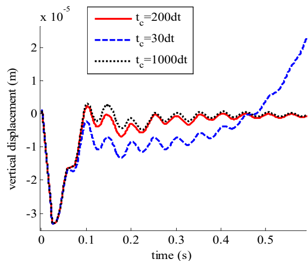
Fig. 20 Vertical displacement time history of point B by three different truncation times
