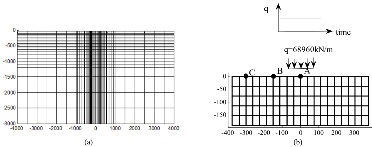
Fig. 15 Used meshes for (a) extended mesh method (b) FEM-SBM analysis
