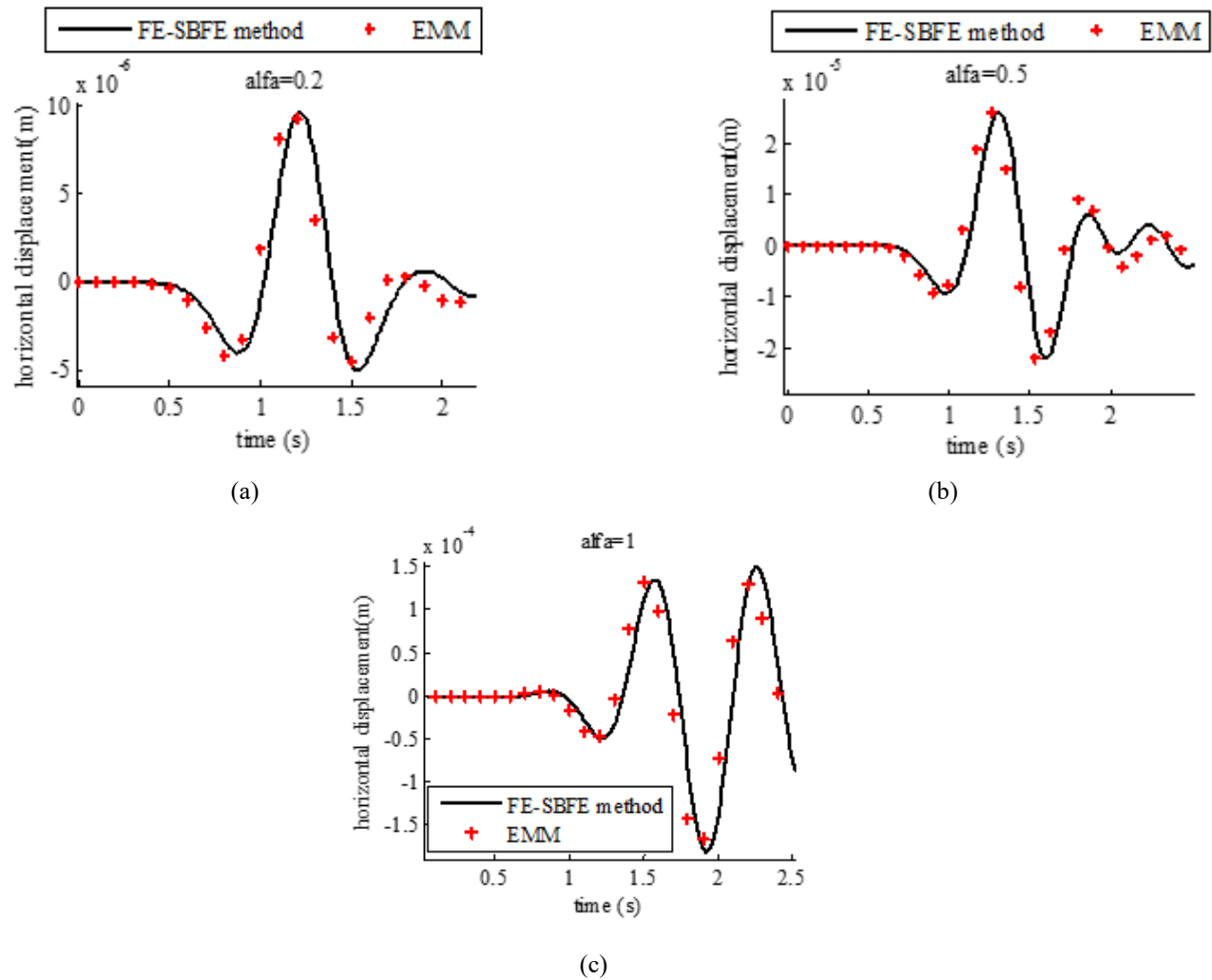
Fig. 14 Displacement time history at point A in non-homogeneous half plane (a) \alpha=0.2 (b) \alpha=0.5 (c) \alpha=1
