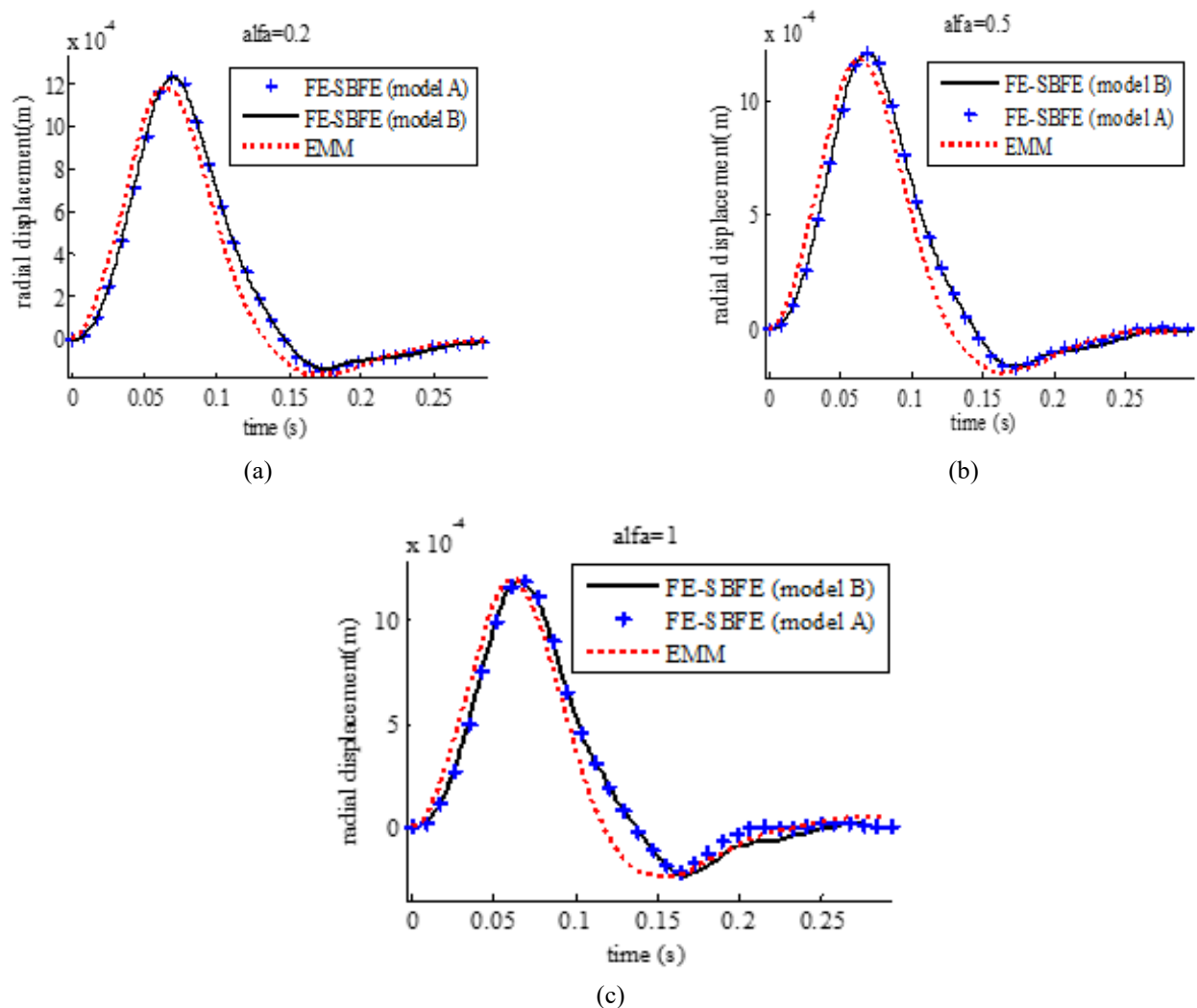
Fig. 9 Radial displacement time history of cavity wall embedded in non-homogenous full plane (a) \alpha=0.2 (b) \alpha=0.5 (c) \alpha=1
