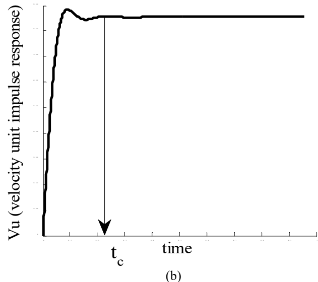
Fig. 2 Diagonal entries of (a) acceleration unit impulse response matrix (b) velocity unit impulse response matrix (Baziar & Song, 2006b)
