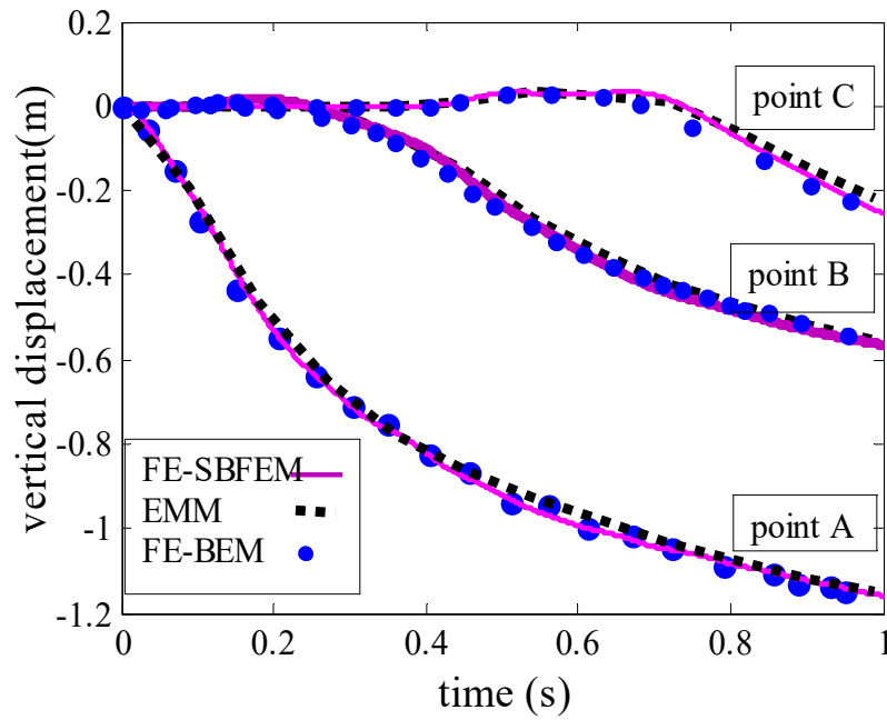
Fig. 16 Displacement time histories for three observation points
