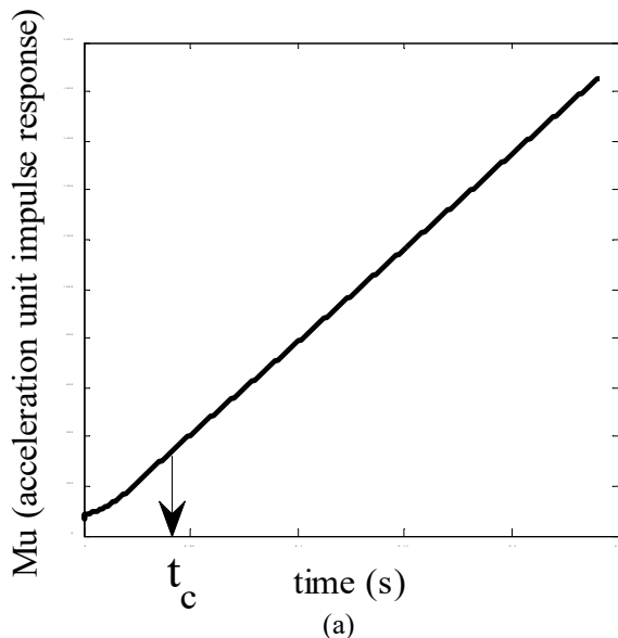
Fig. 2 Diagonal entries of (a) acceleration unit impulse response matrix (b) velocity unit impulse response matrix (Baziar & Song, 2006b)
